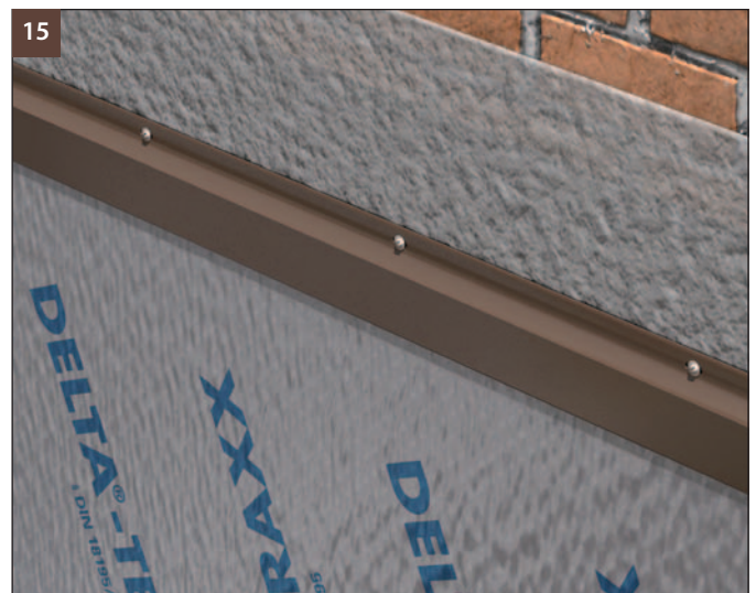
(Fig. 15) Protect the sheet with DELTA ® -NIPPENBAHNE-PROFIL and cover the fastening points.
